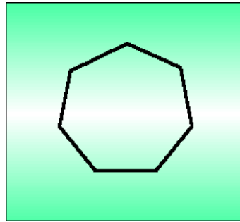
Figure heptagonale
